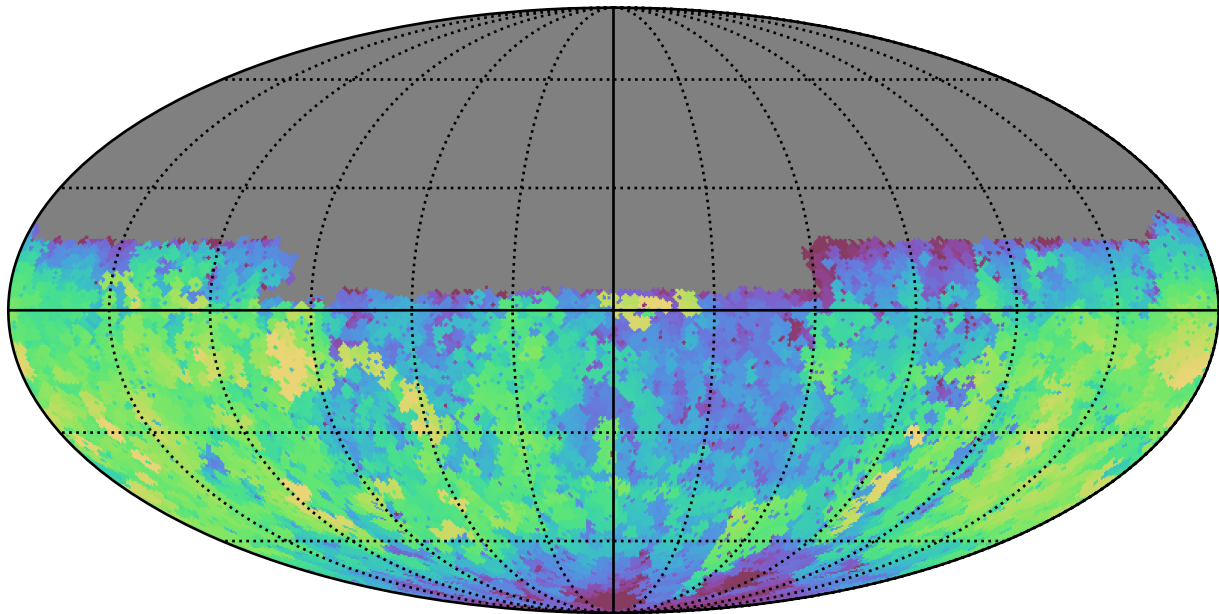
too_5_4v3.4_10yrs Yr 1 u band: Max fiveSigmaDepth
