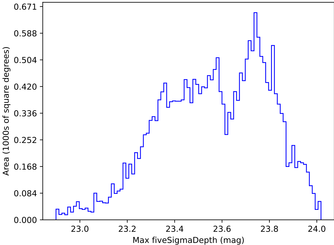
too_5_4v3.4_10yrs Yr 1 u band: Max fiveSigmaDepth
