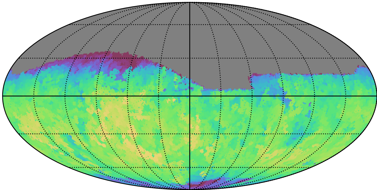
too_5_4v3.4_10yrs Yr 1 r band: Max fiveSigmaDepth
