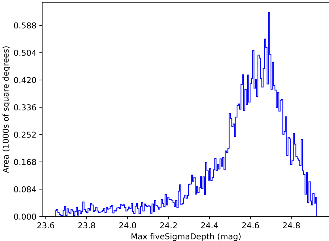
too_5_4v3.4_10yrs Yr 1 r band: Max fiveSigmaDepth
