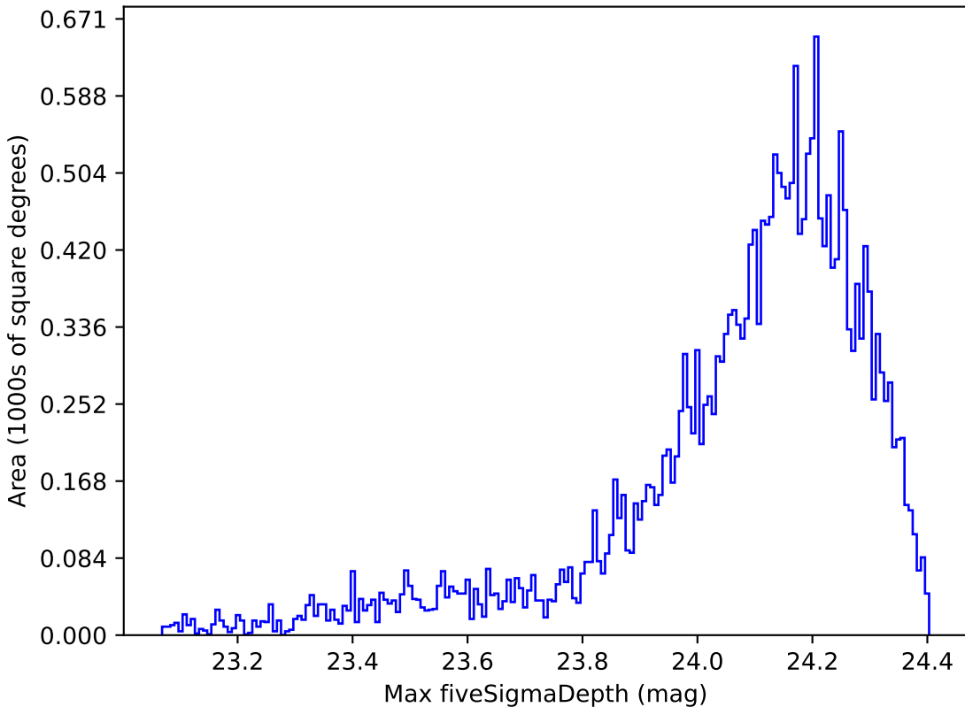
too_5_4v3.4_10yrs Yr 1 i band: Max fiveSigmaDepth
