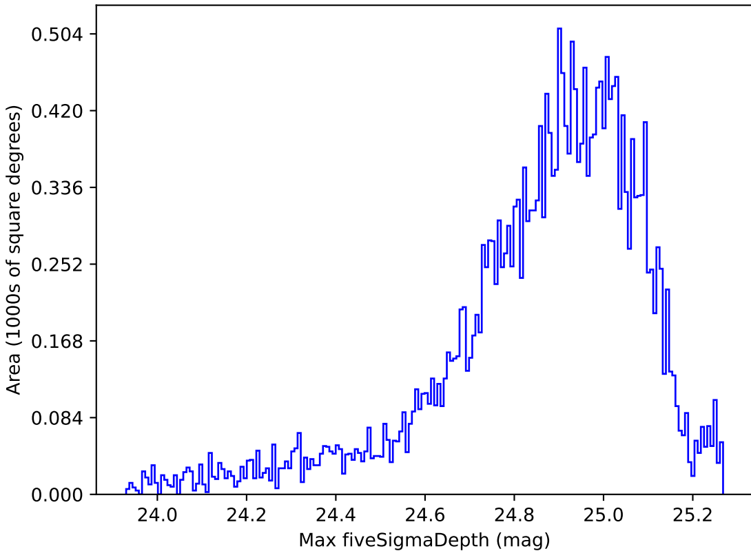
too_5_4v3.4_10yrs Yr 1 g band: Max fiveSigmaDepth
