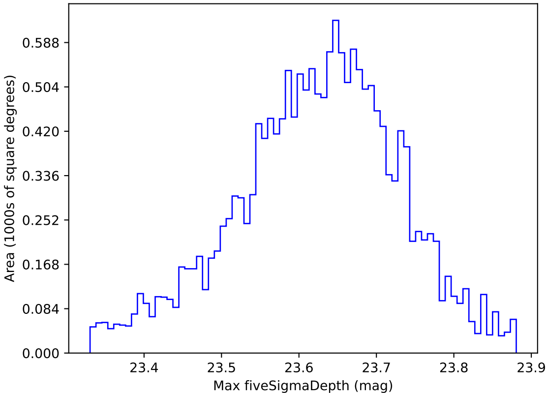
too_5_4v3.4_10yrs WFD z band: Max fiveSigmaDepth
