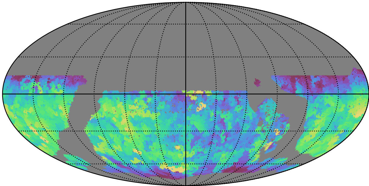
too_5_4v3.4_10yrs WFD u band: Max fiveSigmaDepth
