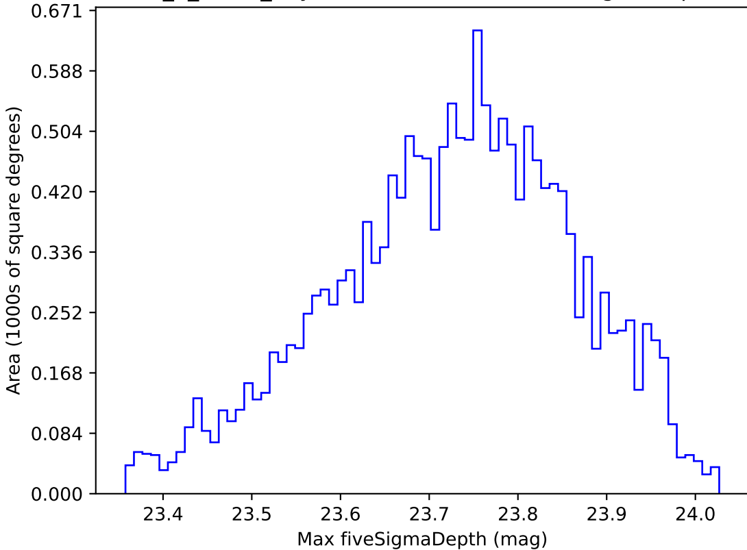
too_5_4v3.4_10yrs WFD u band: Max fiveSigmaDepth
