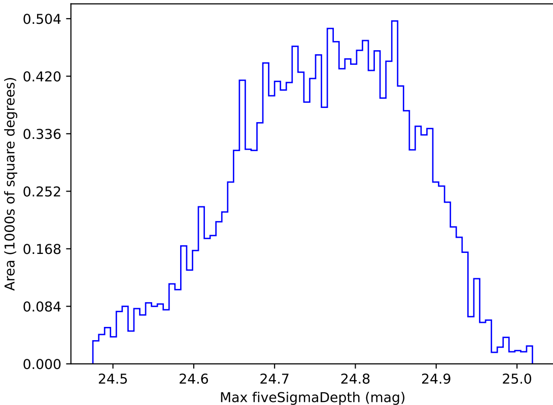
too_5_4v3.4_10yrs WFD r band: Max fiveSigmaDepth
