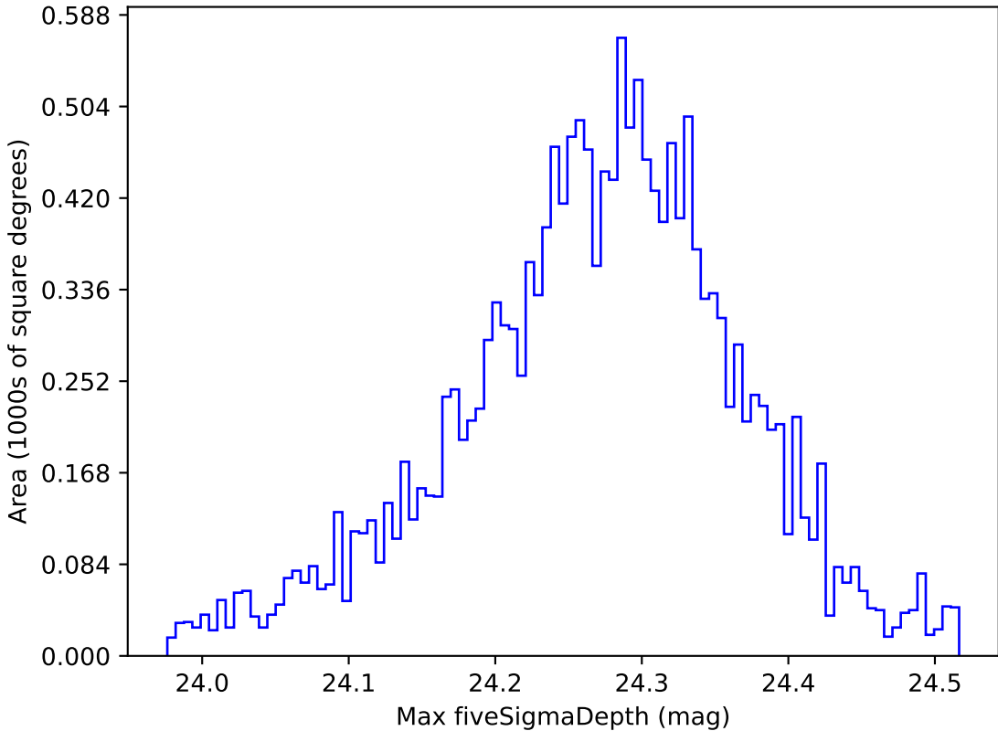
too_5_4v3.4_10yrs WFD i band: Max fiveSigmaDepth
