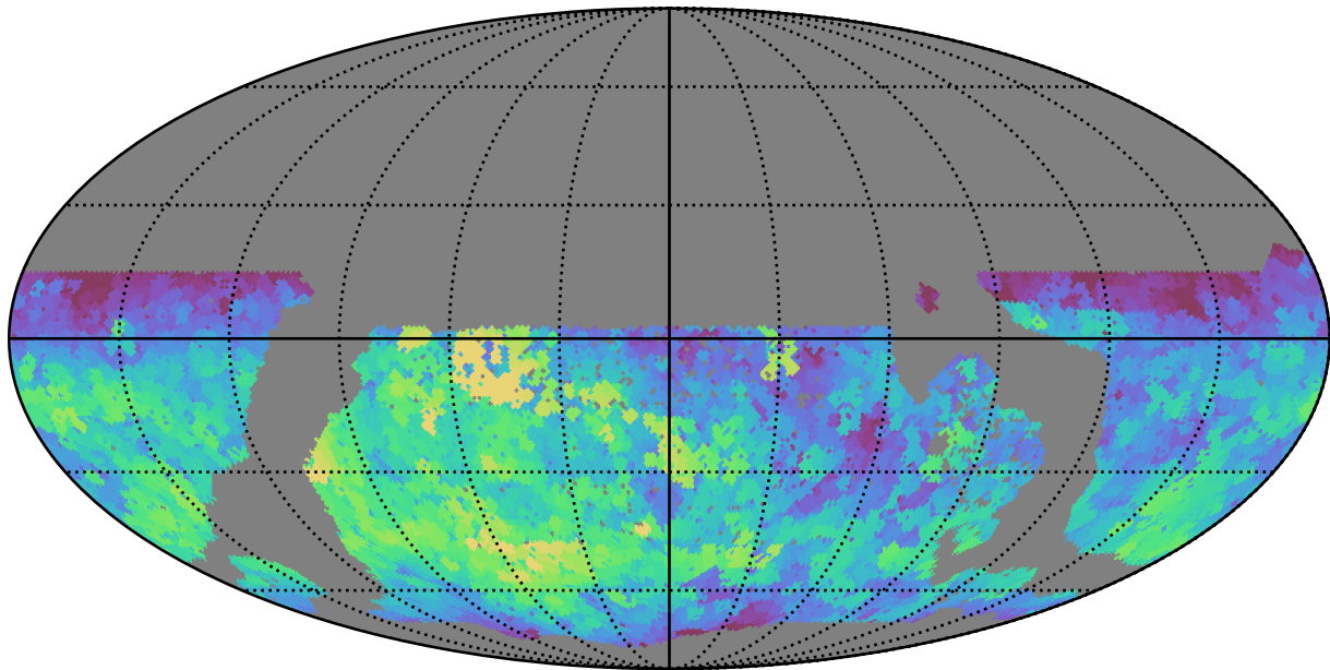
too_5_4v3.4_10yrs WFD g band: Max fiveSigmaDepth
