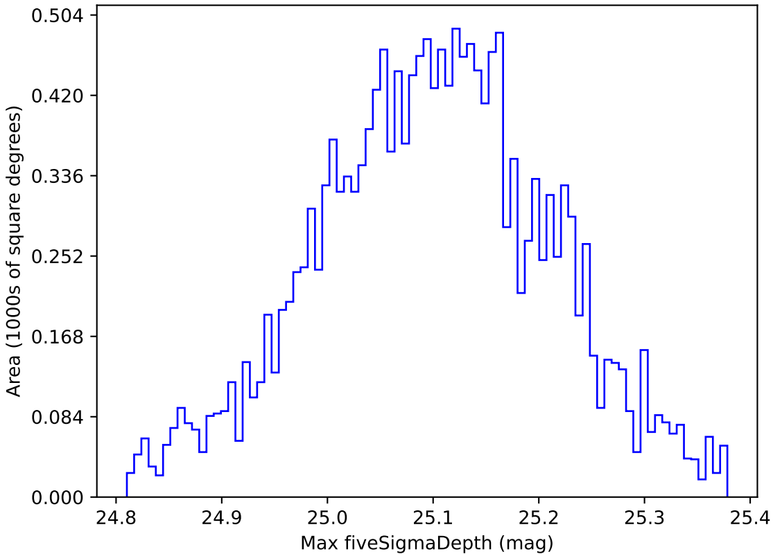
too_5_4v3.4_10yrs WFD g band: Max fiveSigmaDepth
