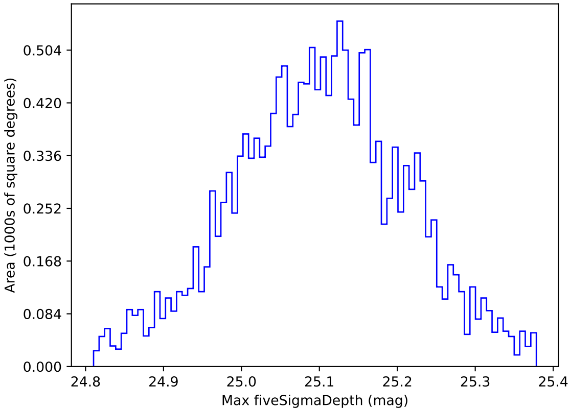
too_5_4v3.4_10yrs WFD all bands: Max fiveSigmaDepth
