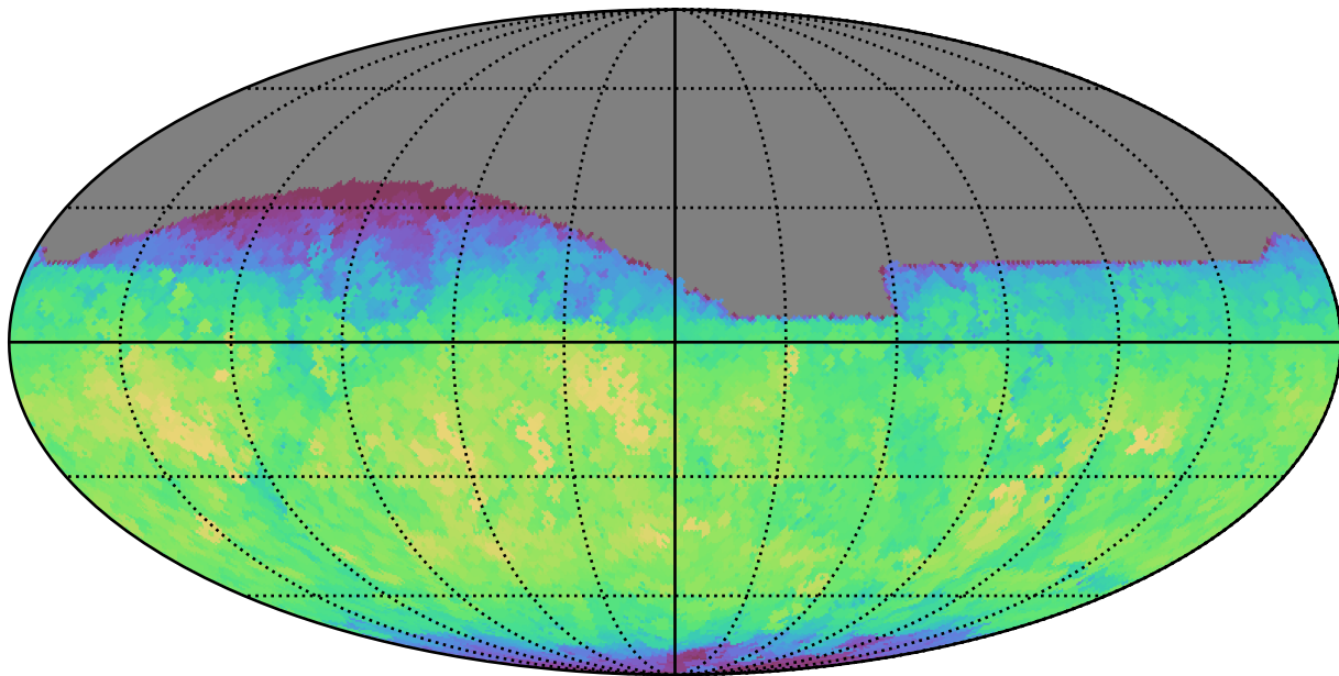
too_5_4v3.4_10yrs All sky z band: Max fiveSigmaDepth
