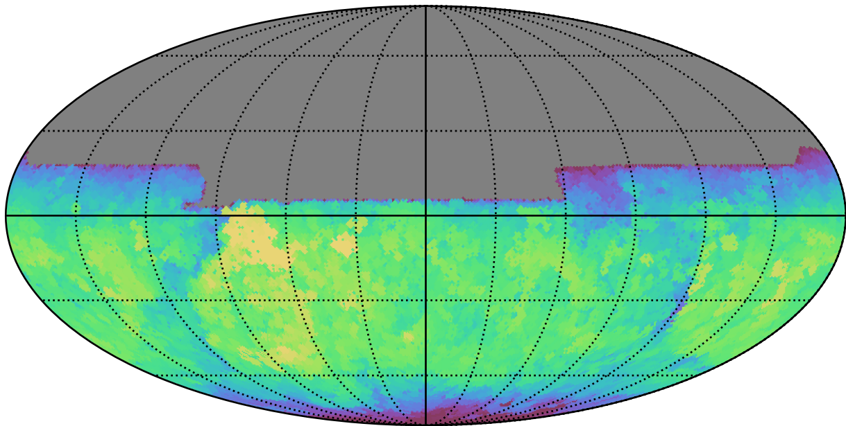
too_5_4v3.4_10yrs All sky y band: Max fiveSigmaDepth
