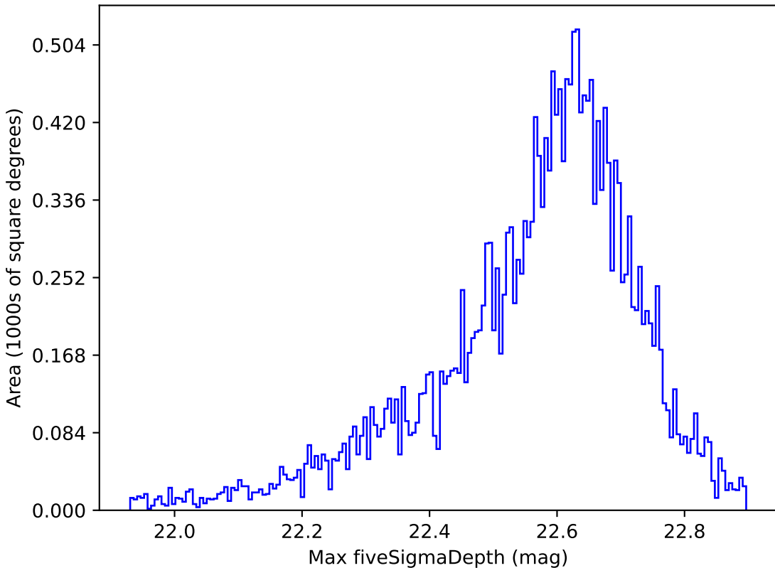
too_5_4v3.4_10yrs All sky y band: Max fiveSigmaDepth
