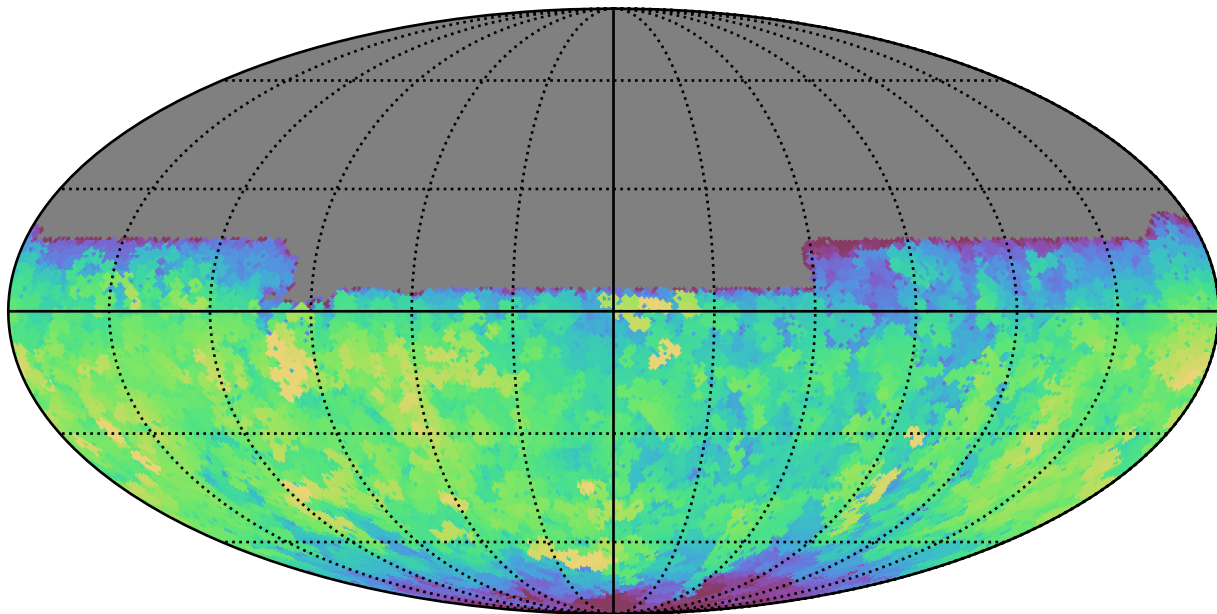
too_5_4v3.4_10yrs All sky u band: Max fiveSigmaDepth
