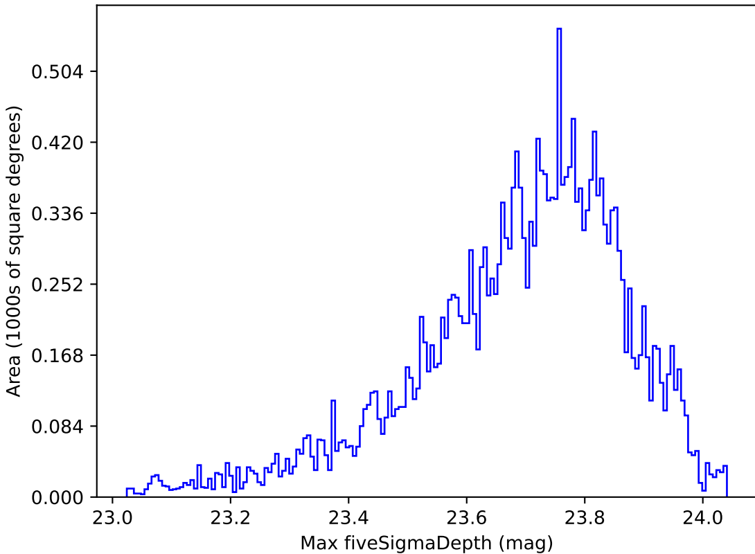
too_5_4v3.4_10yrs All sky u band: Max fiveSigmaDepth
