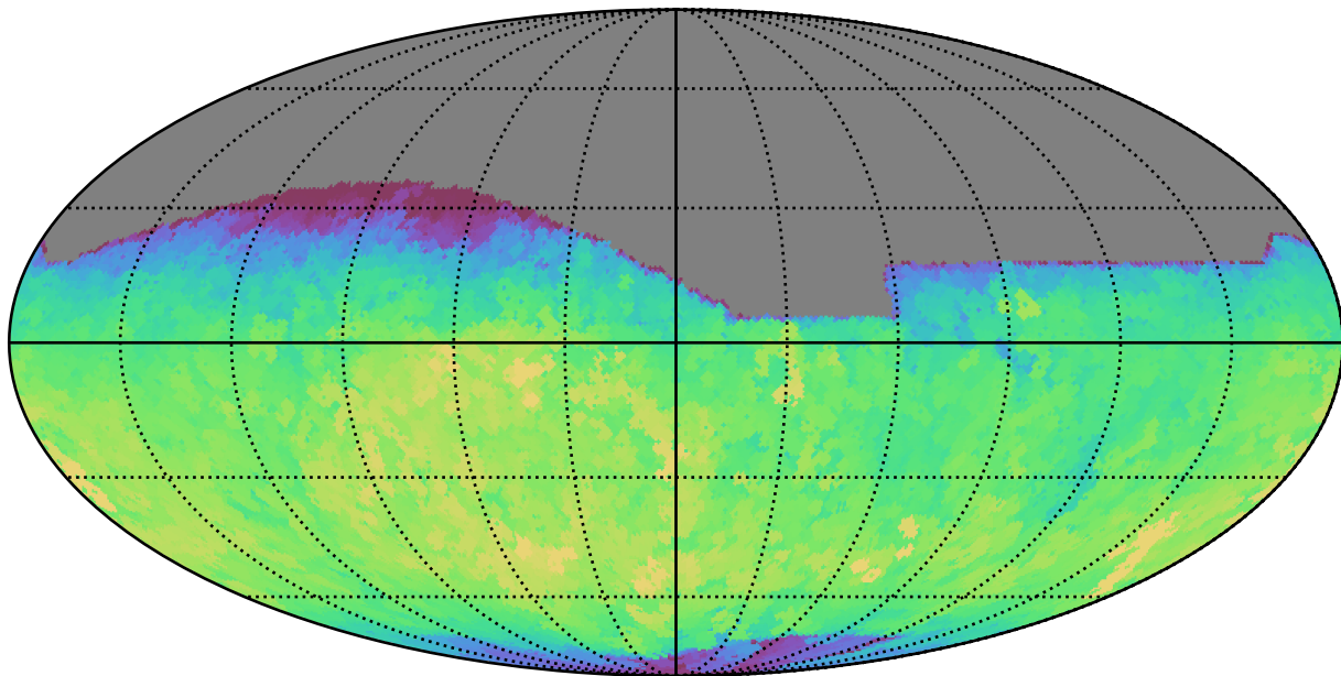
too_5_4v3.4_10yrs All sky r band: Max fiveSigmaDepth
