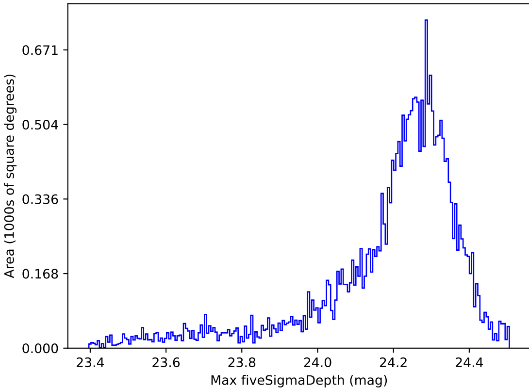
too_5_4v3.4_10yrs All sky i band: Max fiveSigmaDepth
