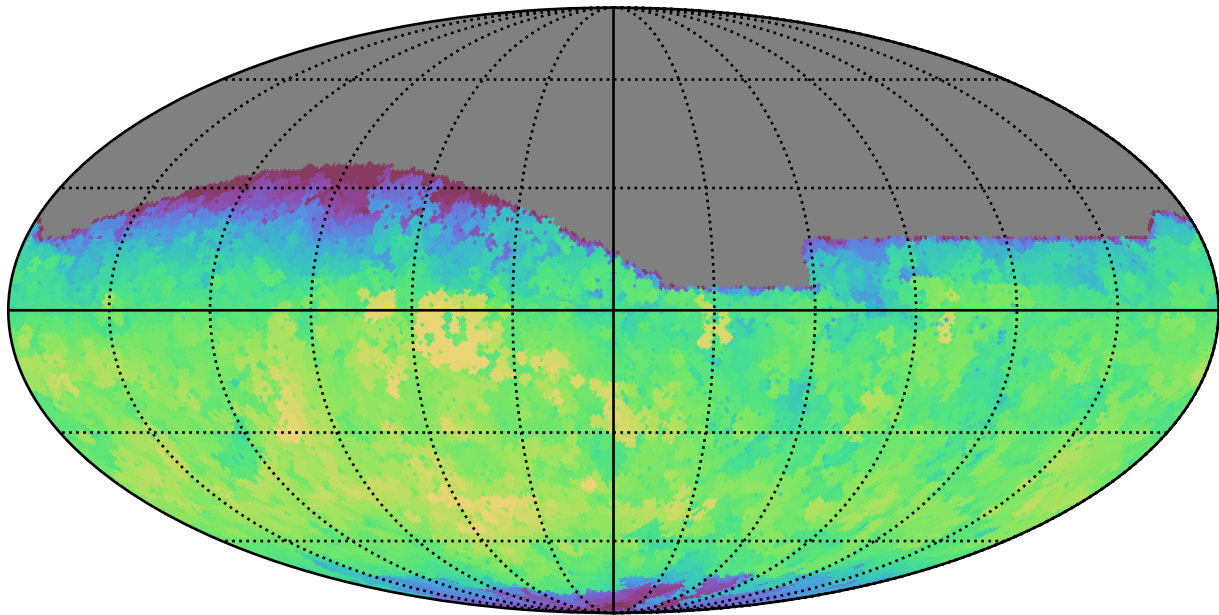
too_5_4v3.4_10yrs All sky g band: Max fiveSigmaDepth
