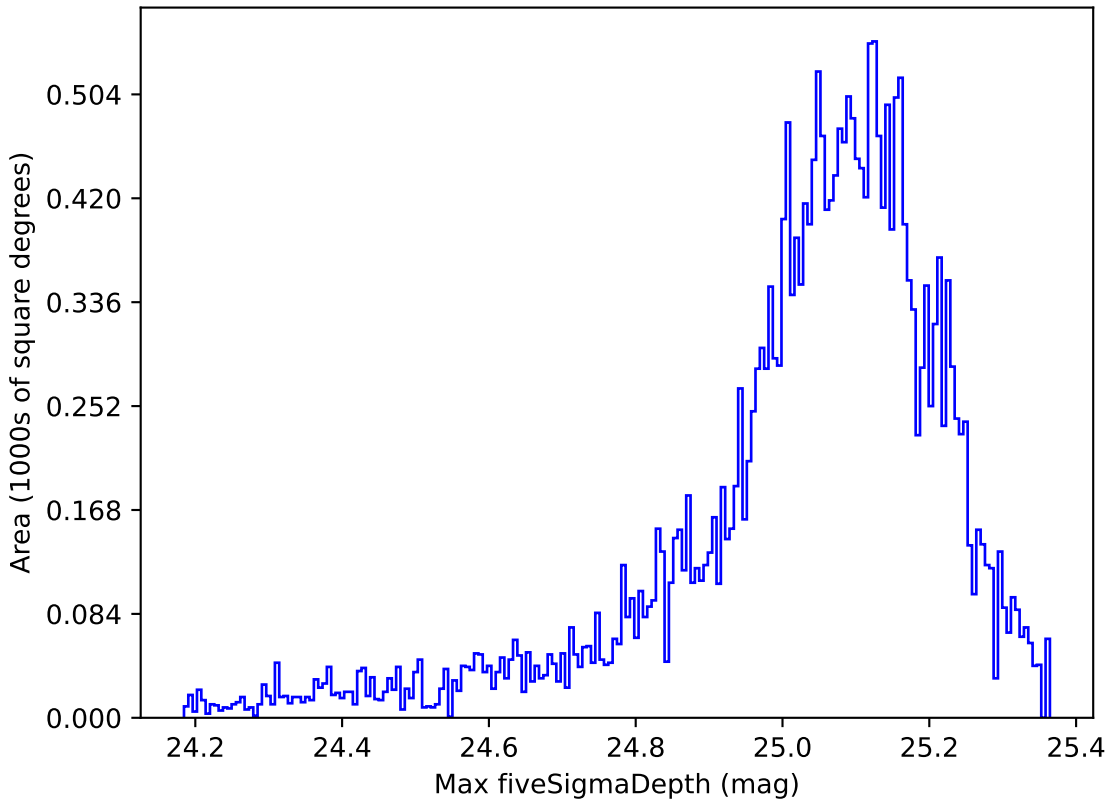
too_5_4v3.4_10yrs All sky g band: Max fiveSigmaDepth
