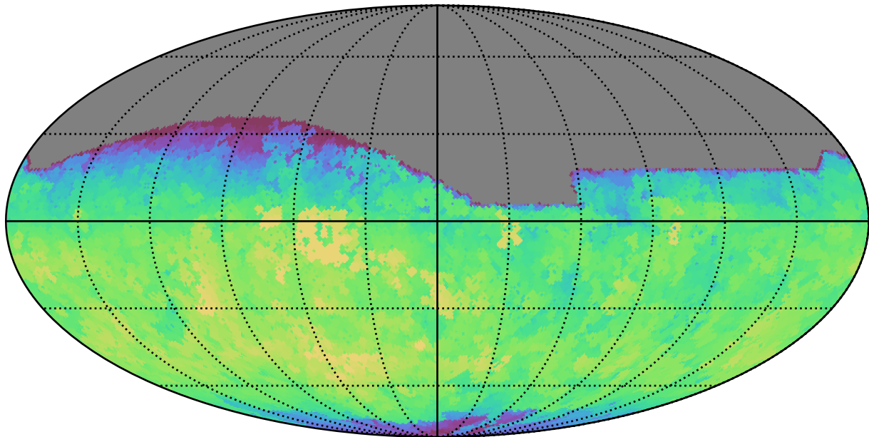
too_5_4v3.4_10yrs All sky all bands: Max fiveSigmaDepth
