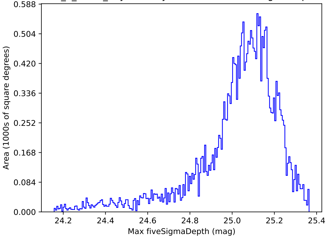
too_5_4v3.4_10yrs All sky all bands: Max fiveSigmaDepth
