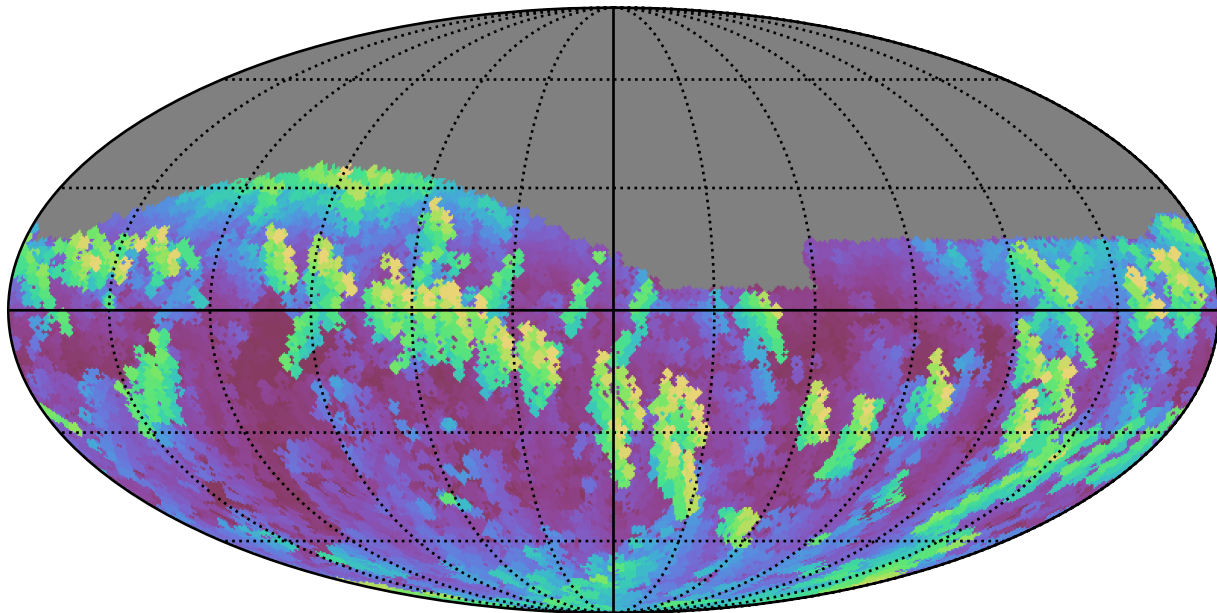
too_5_4v3.4_10yrs Yr 1 z band: Max airmass
