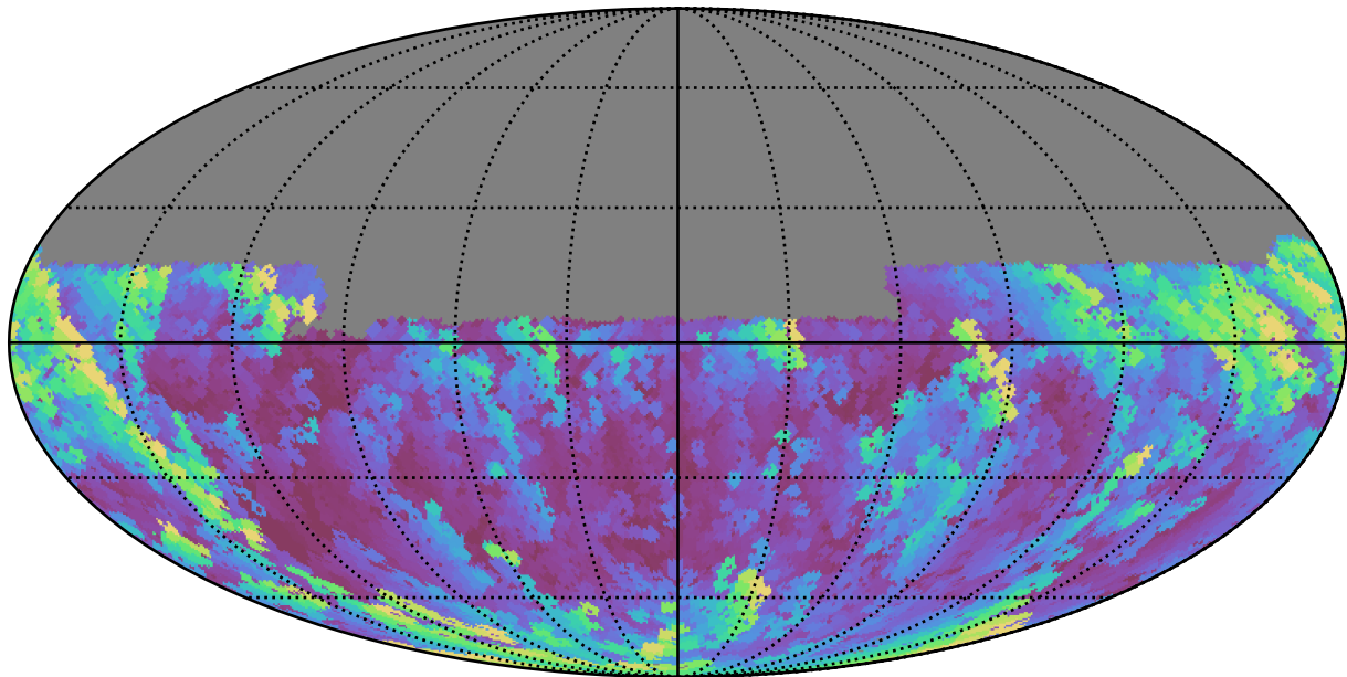
too_5_4v3.4_10yrs Yr 1 y band: Max airmass
