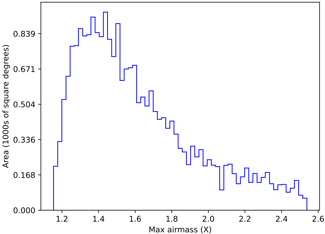
too_5_4v3.4_10yrs Yr 1 y band: Max airmass
