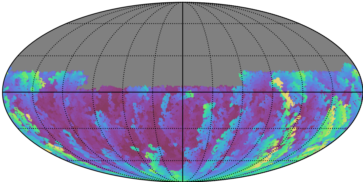
too_5_4v3.4_10yrs Yr 1 u band: Max airmass
