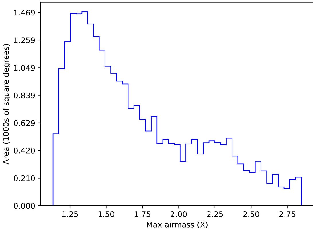
too_5_4v3.4_10yrs Yr 1 i band: Max airmass
