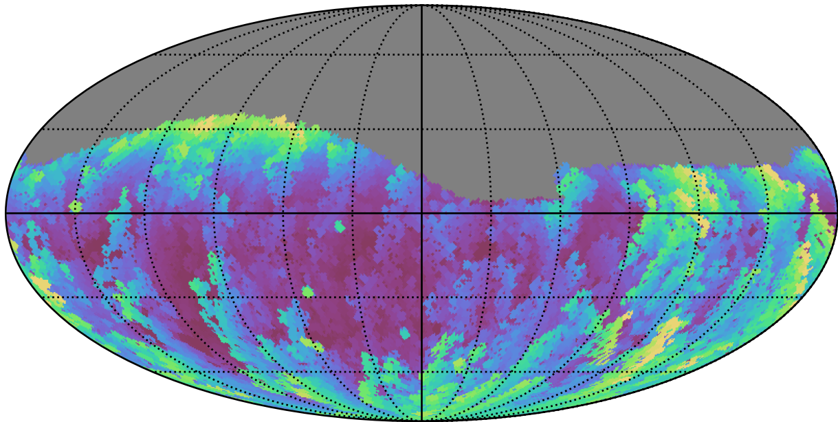
too_5_4v3.4_10yrs Yr 1 g band: Max airmass
