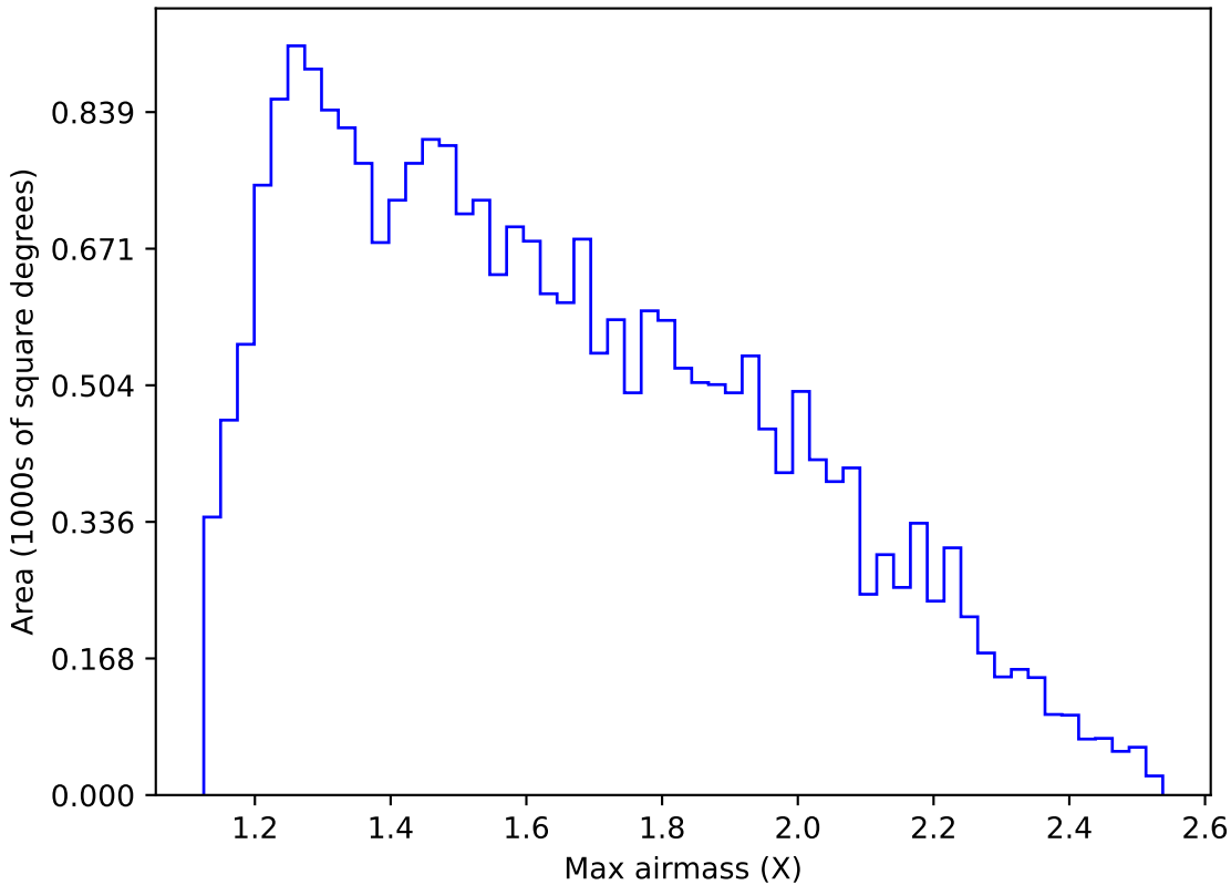
too_5_4v3.4_10yrs Yr 1 g band: Max airmass
