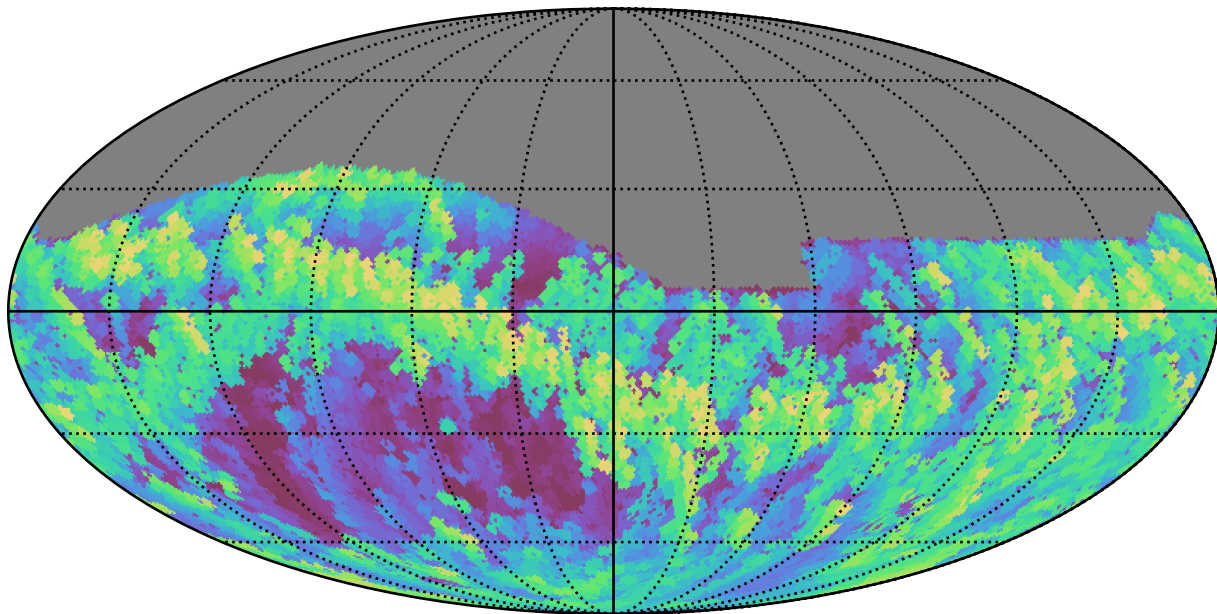
too_5_4v3.4_10yrs Yr 1 all bands: Max airmass
