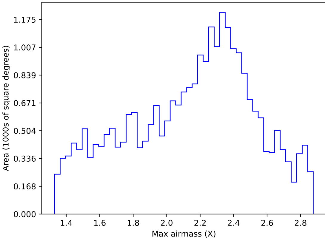
too_5_4v3.4_10yrs Yr 1 all bands: Max airmass
