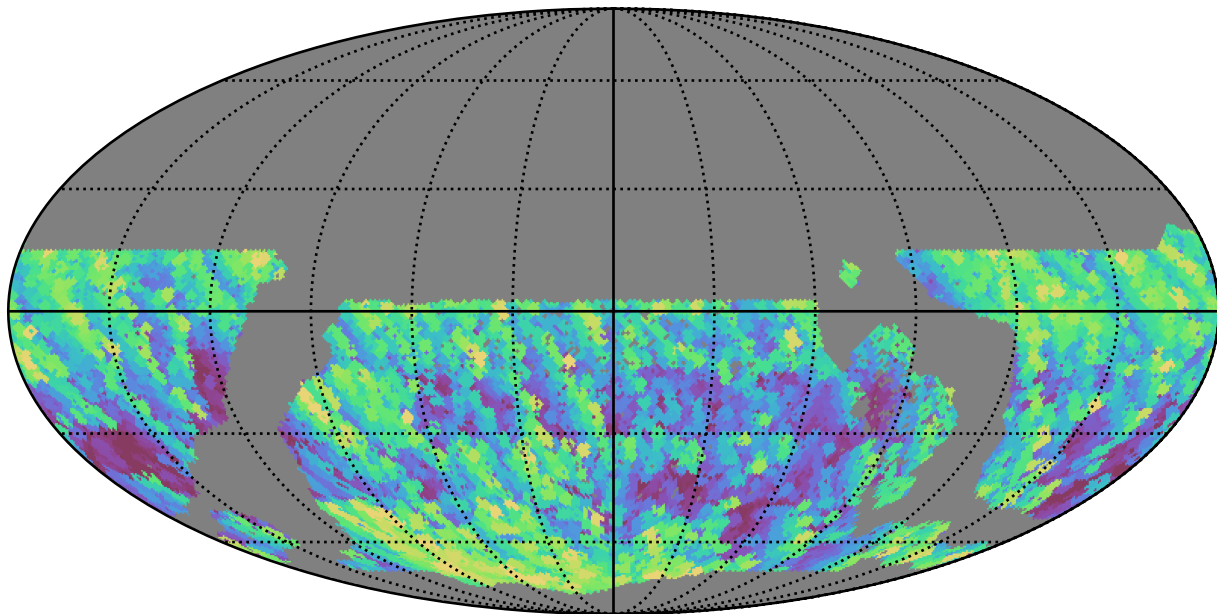
too_5_4v3.4_10yrs WFD y band: Max airmass
