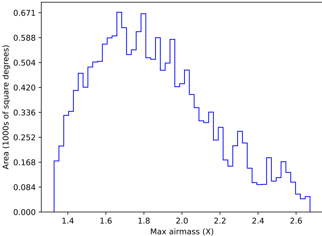
too_5_4v3.4_10yrs WFD u band: Max airmass
