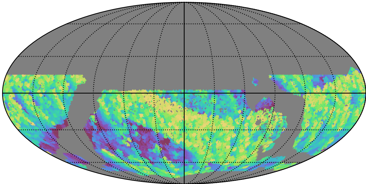
too_5_4v3.4_10yrs WFD i band: Max airmass
