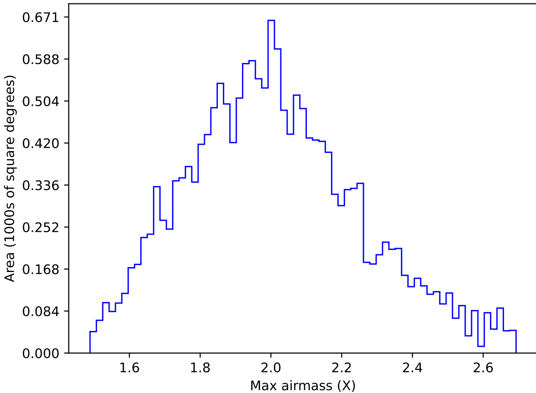
too_5_4v3.4_10yrs WFD g band: Max airmass
