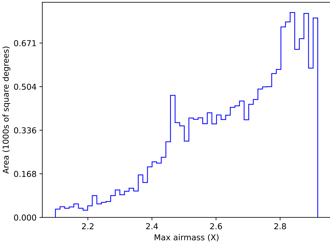
too_5_4v3.4_10yrs WFD all bands: Max airmass
