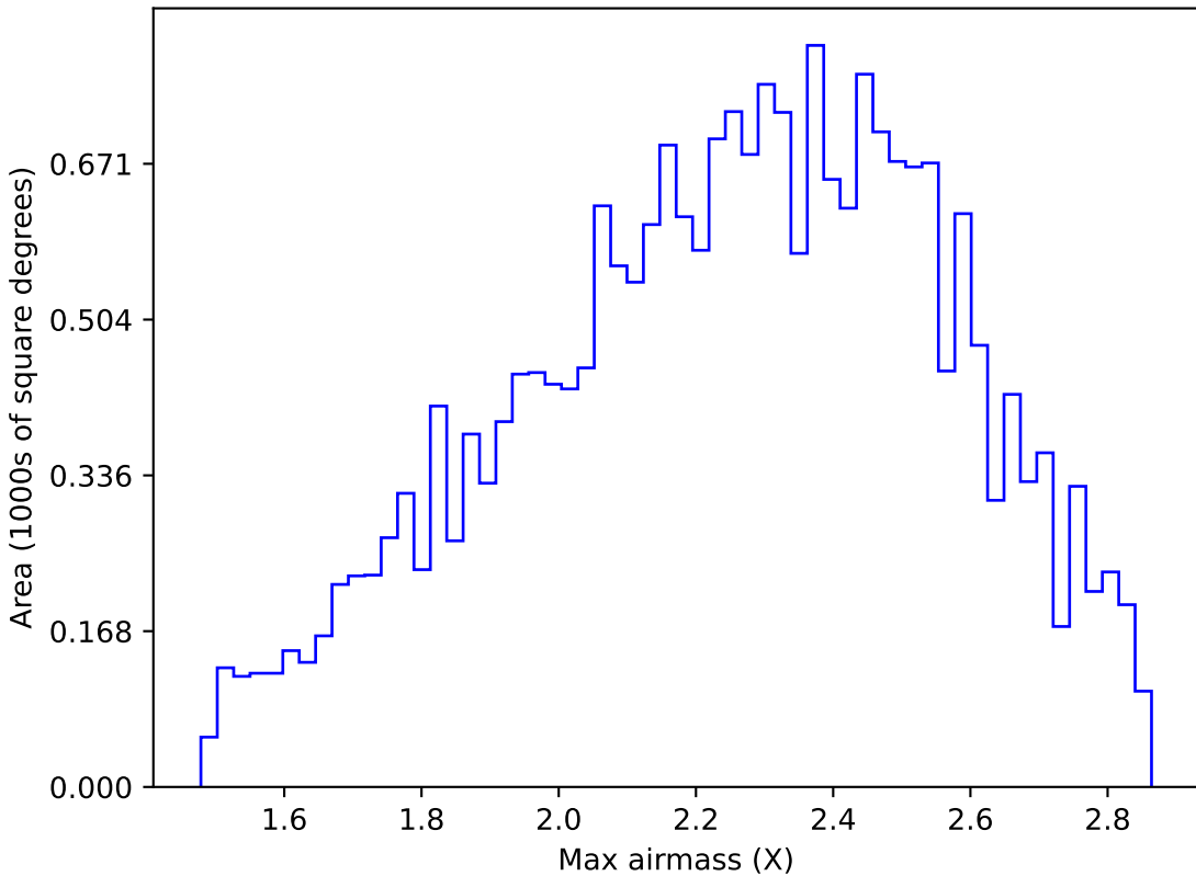
too_5_4v3.4_10yrs All sky y band: Max airmass
