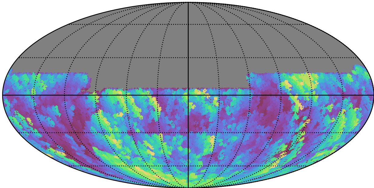
too_5_4v3.4_10yrs All sky u band: Max airmass
