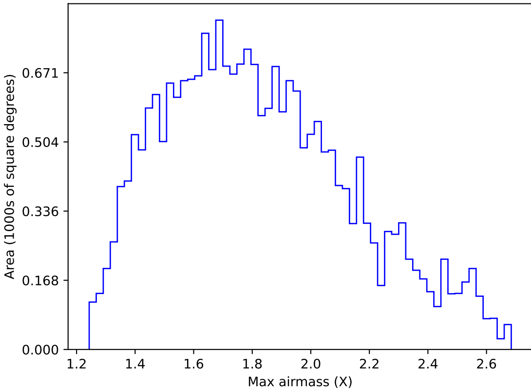
too_5_4v3.4_10yrs All sky u band: Max airmass
