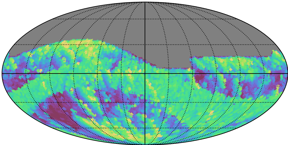
too_5_4v3.4_10yrs All sky r band: Max airmass
