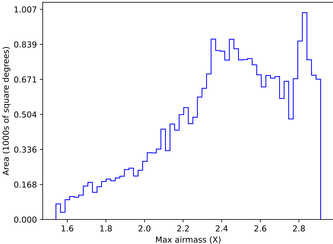
too_5_4v3.4_10yrs All sky i band: Max airmass
