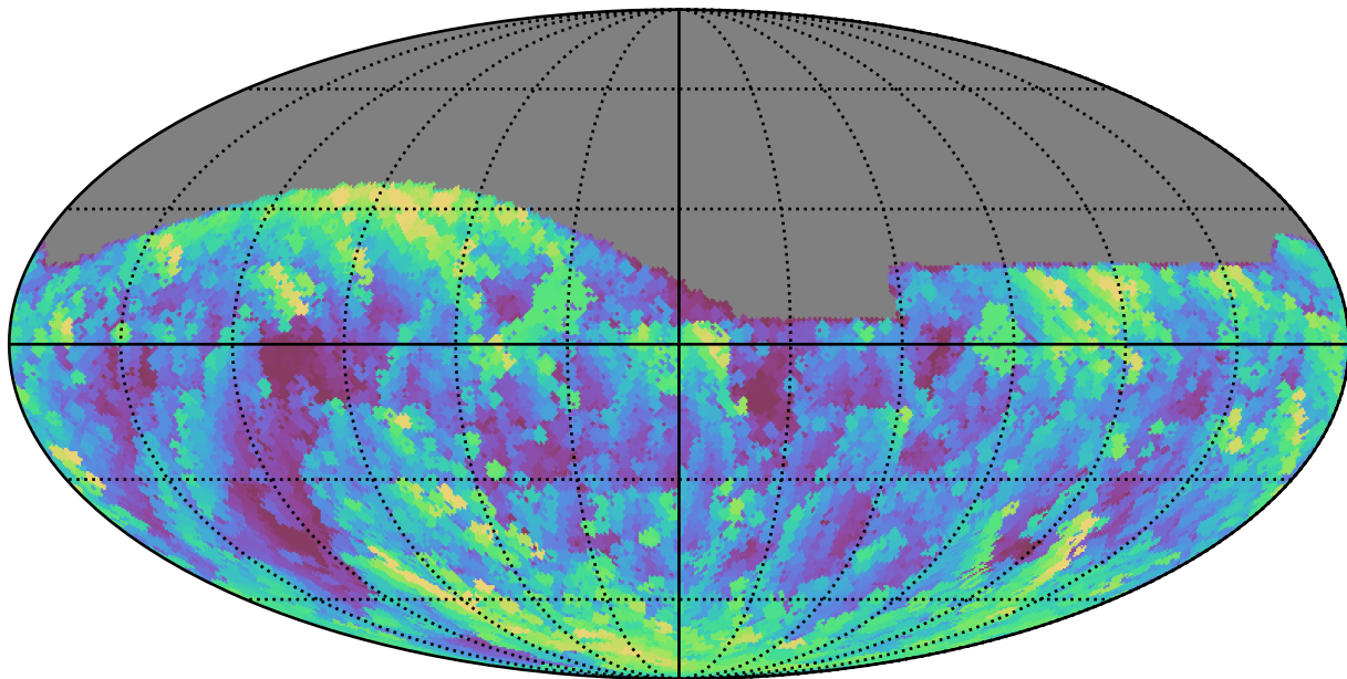
too_5_4v3.4_10yrs All sky g band: Max airmass
