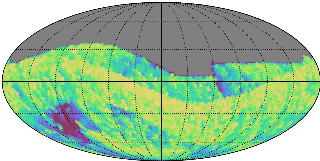
too_5_4v3.4_10yrs All sky all bands: Max airmass
