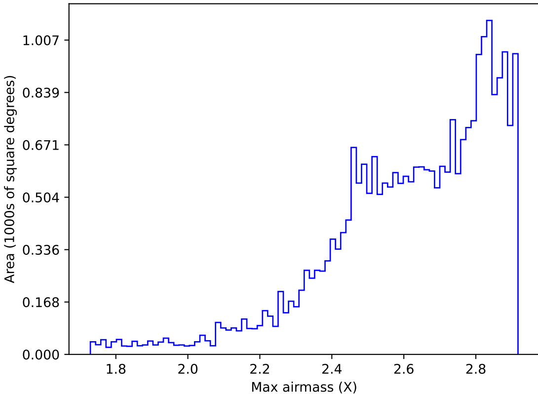
too_5_4v3.4_10yrs All sky all bands: Max airmass
