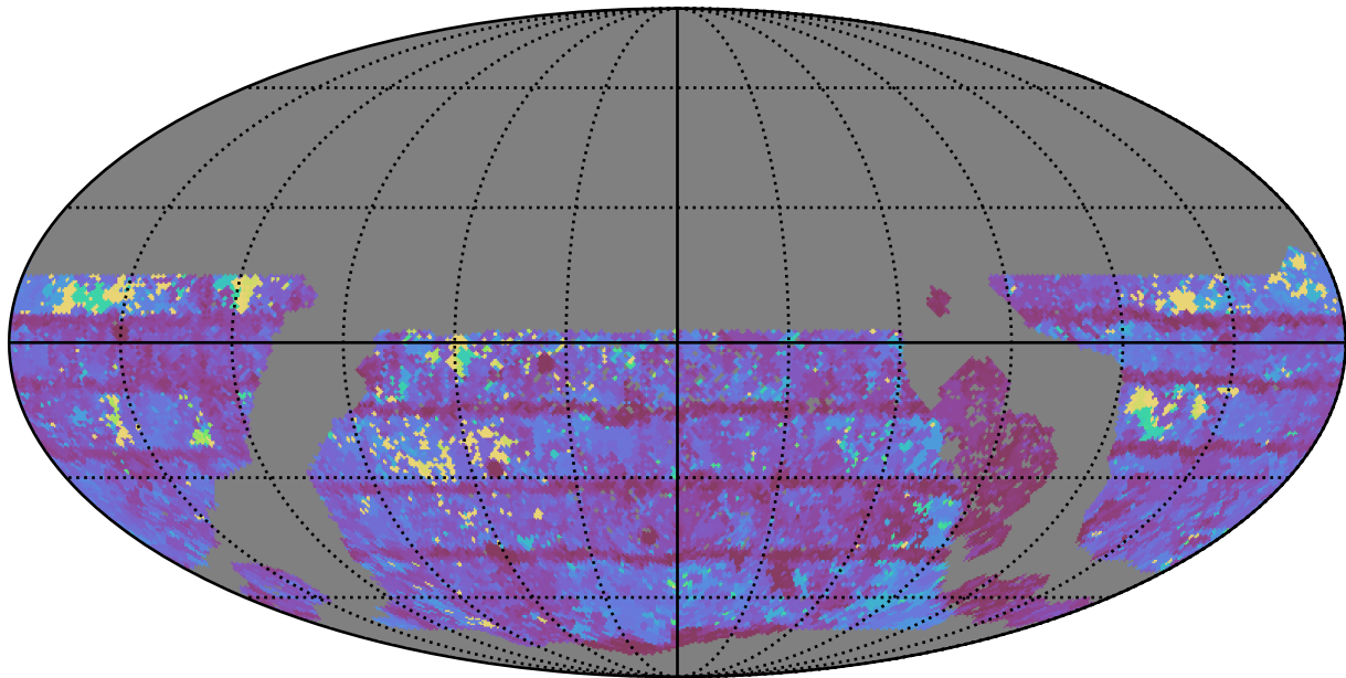
too_5_4v3.4_10yrs WFD z band: Max Inter-Night Gap
