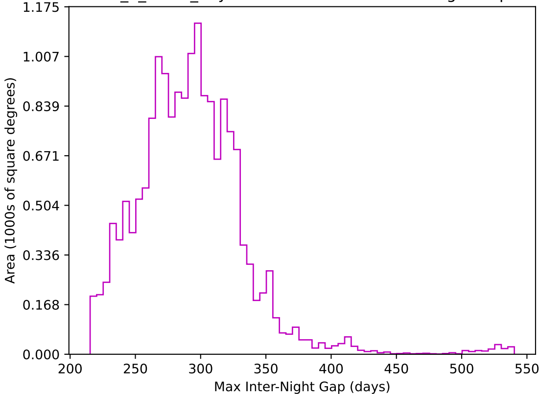
too_5_4v3.4_10yrs WFD z band: Max Inter-Night Gap
