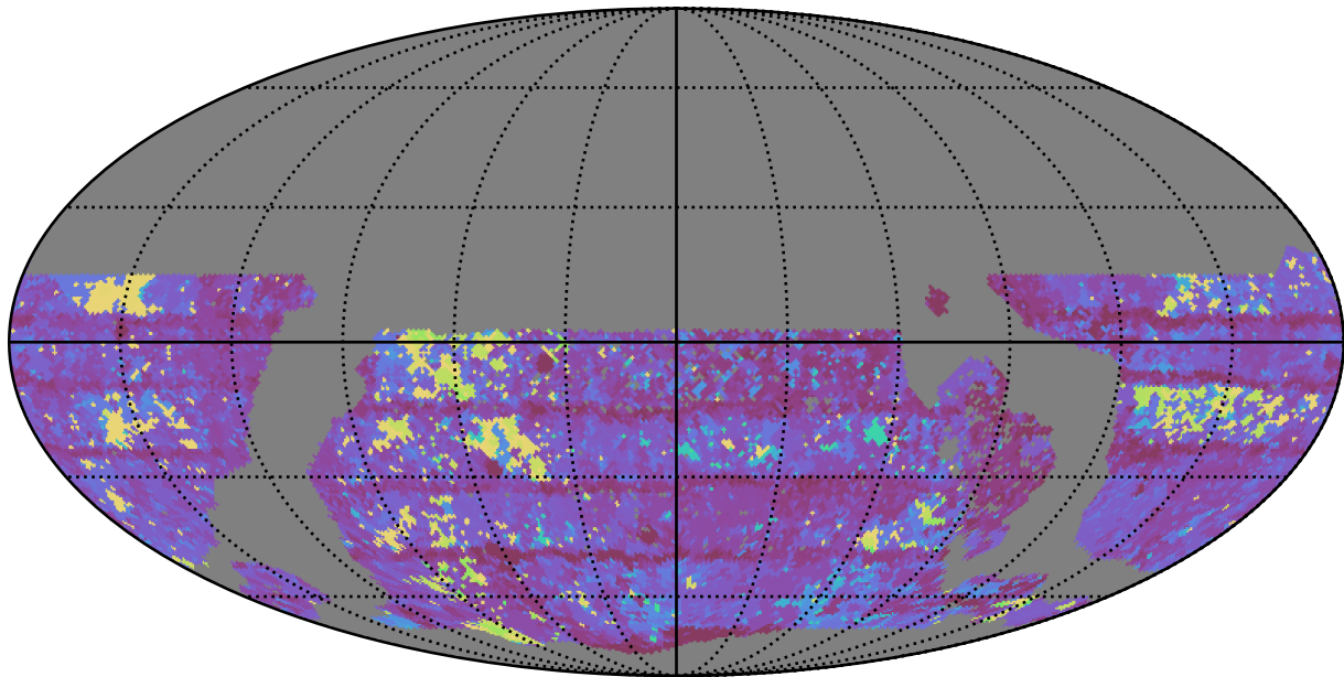
too_5_4v3.4_10yrs WFD y band: Max Inter-Night Gap
